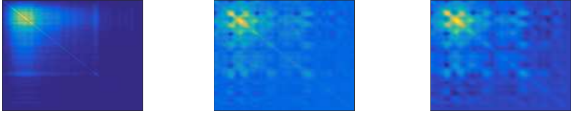
(a) True covariance. (b) Initial covariance estimate. (c) Blurred covariance estimate.
