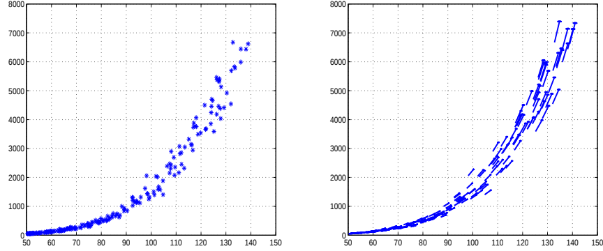
Figure 1: Left: Sample points of 2D with \sigma = 0.2 . Right: Gradients estimated by UM.
